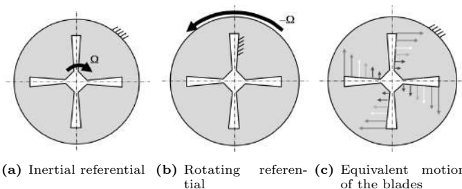
Figure 5: Single rotating frame of reference. In [19].
