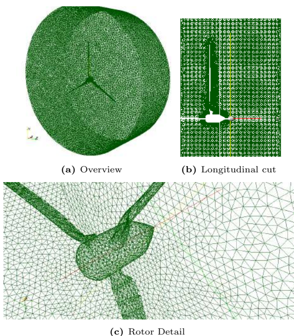
Figure 9: Final fluid mesh details.
