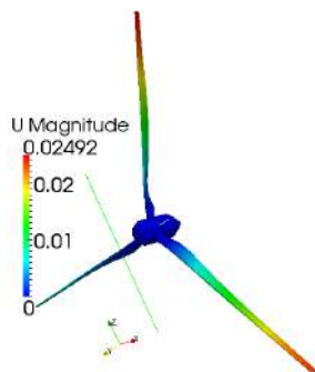
Figure 14: Displacement in the blades due to the flow.
