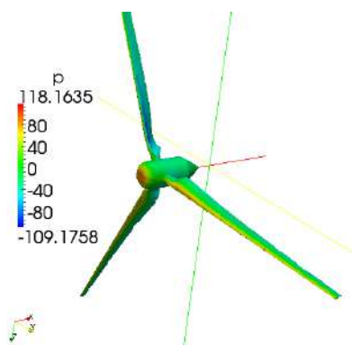
Figure 11: Pressure on the rotor.
