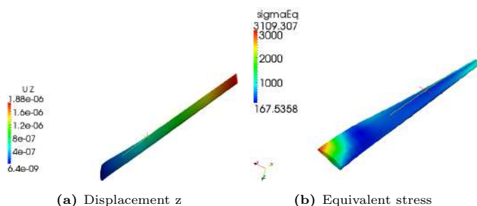
Figure 13: Simulation of the blade using stressedFoam .
