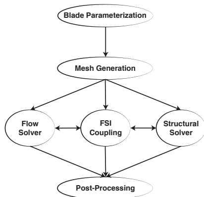
Figure 1: Schematic of WT aero-structural blade analysis.
