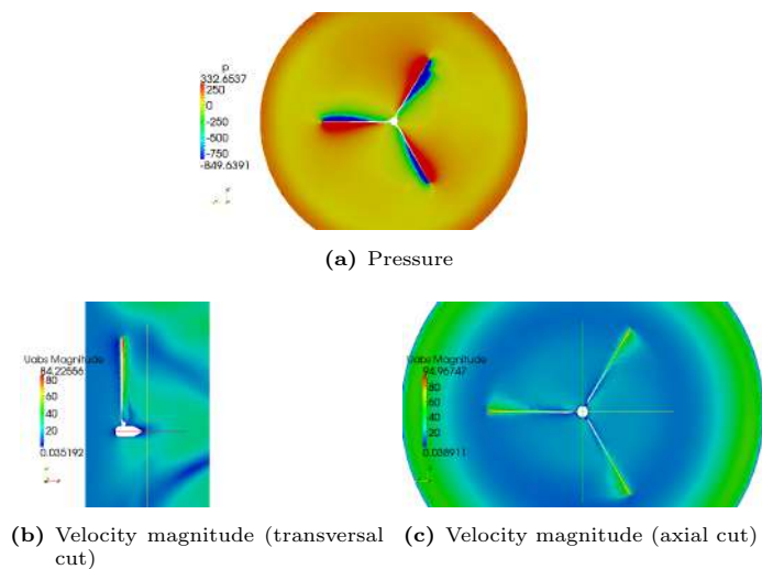
Figure 15: Flow results on the FSI simulation of the HAWT blades.
