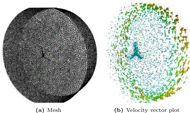
Figure 6: SRF simulation of the rotor.
