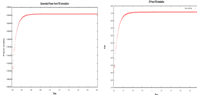
(a) Power, converged at 4.24\text{MW} (b) C_p , converged at 0.46
