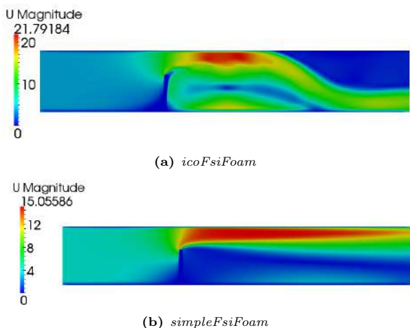
Figure 3: Velocity around a 2D beam using FSI solvers.
