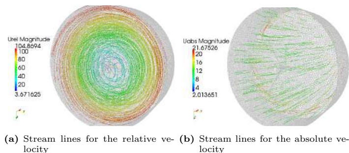
Figure 10: Final results for the flow simulations.
