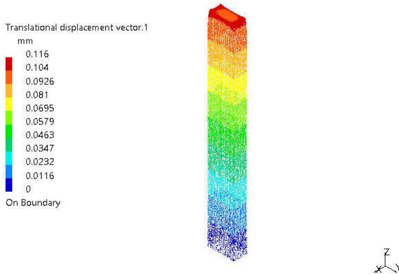
Figure 6.4: Deformation of the specimen under the selected loading.
