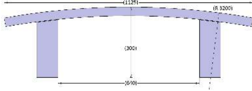
Figure 2: Bumper geometry measurements
