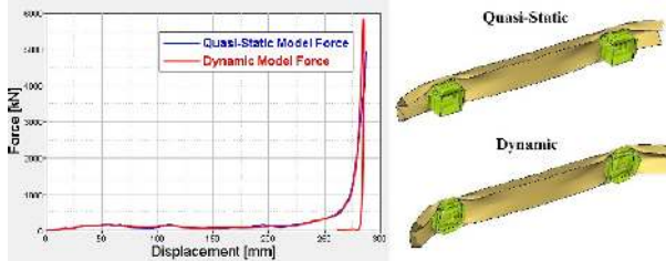
Figure 6: Comparison between quasi-static and dynamic tests
