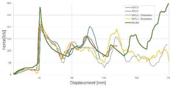
Figure 5: Experimental results vs quasi-static model
