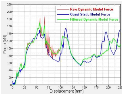
Figure 7: Comparison between quasi-static and CFC 1000 filtered dynamic test
