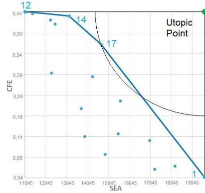
Figure 9: Pareto set of first iteration (each point corresponds to a different geometry)
