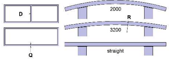
Figure 11: Parameters that were changed in the second iteration
