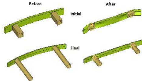
Figure 14: Comparison between the initial geometry and the resultant of the optimization process
