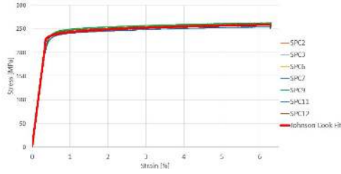
Figure 3: Johnson Cook material model curve compared with tensile test results
