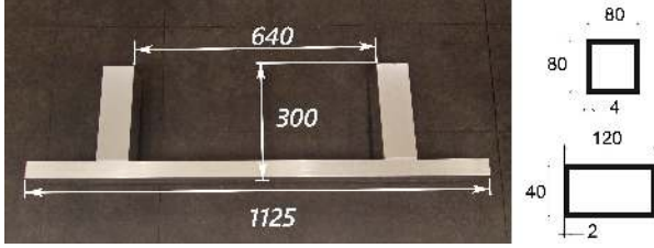
Figure 4: Compression procedure specimen measurements
