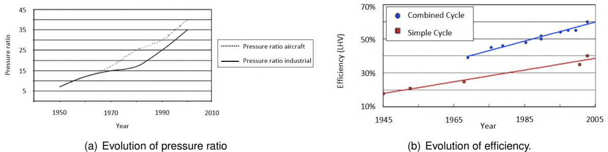
Figure 3.1: Evolution of pressure ratio and thermal efficiency over the years [23].
