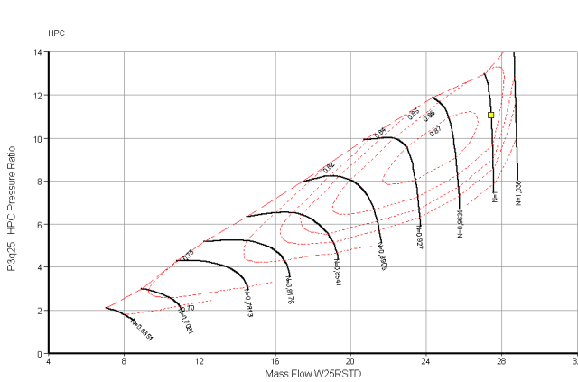
(a) Indetermination of flow/pressure ratio values in a compressor map.
