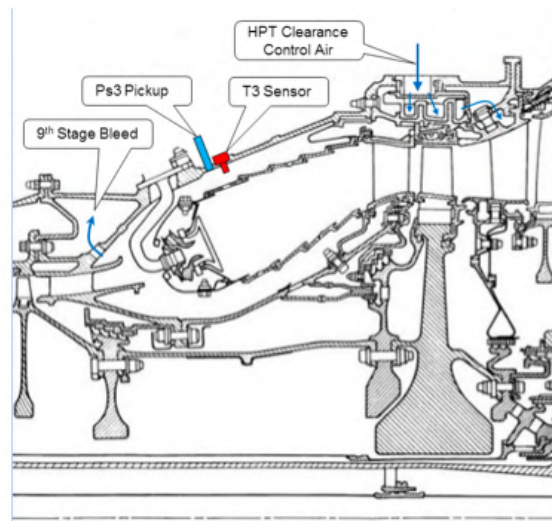
Figure 4.3: Location of T3 and Ps3 sensors [37].
