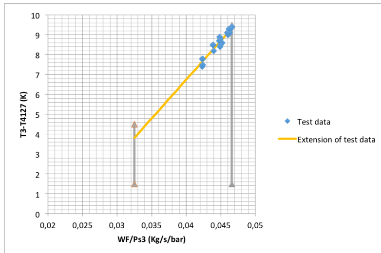
Figure 4.4: Difference between measured T3 and T4127.
