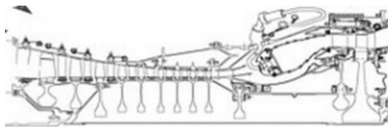
Figure 6.1: CFM56-3 high pressure compressor [22].
