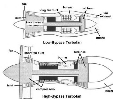
Figure 3.2: Low by-pass and high by-pass engines [25].
