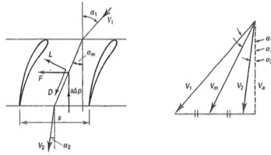
Figure 6.2: Forces and velocities acting on a cascade [26].
