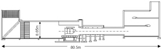
Figure 2.3: TAP test cell [12].
