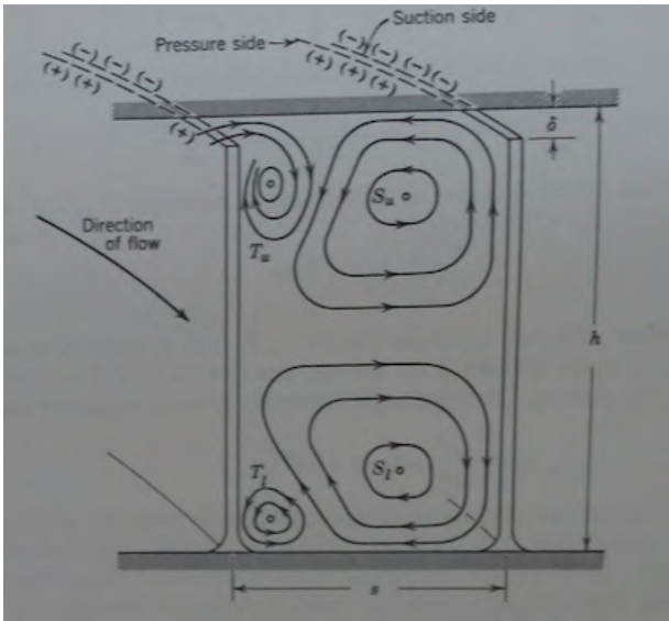
Figure 6.8: Vortex pattern in a cascade [50].
