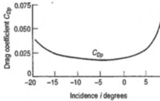
Figure 6.3: Profile drag coefficient versus incidence angle i [50].
