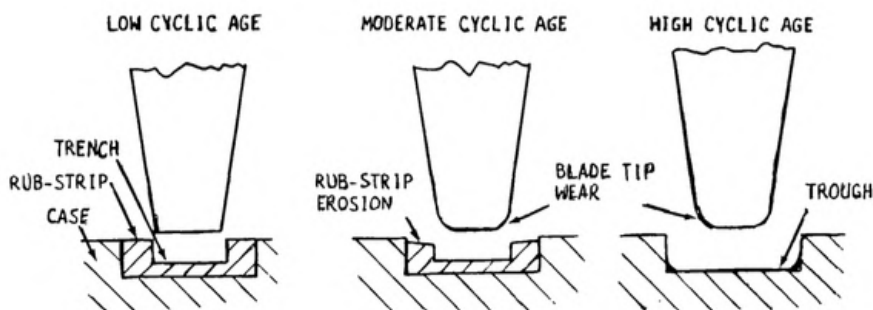
Figure 3.7: Evolution of erosion on HPC blades and rub-strips [33].
