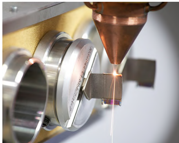
Figure 5.1: HPC blade chord length restoration [47].
