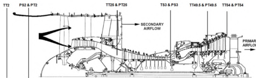
Figure 2.5: Position of thermodynamic stations in CFM56-3 [18].
