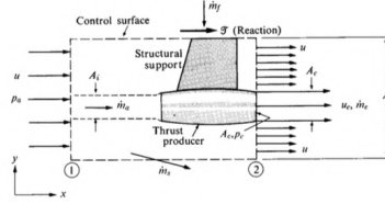
Figure 3.3: Generalized thrust-producing device [30].
