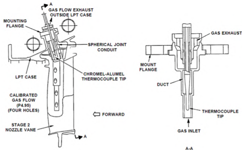
Figure 4.8: Schematic of the TT495 sensor [18].
