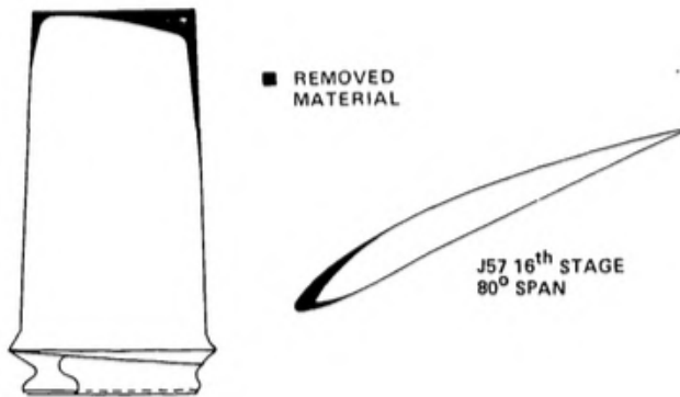
(a) Erosion on a compressor blade
