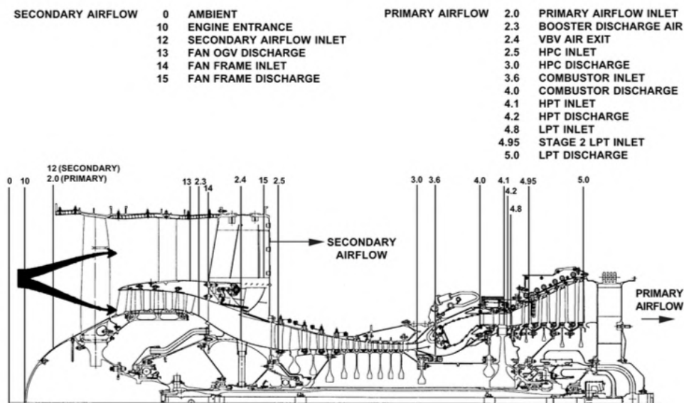
Figure 4.2: CFM56-3 thermodynamic stations [17].
