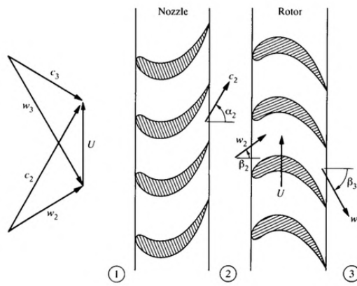
Figure 6.4: Degree of reaction of 50% [30].
