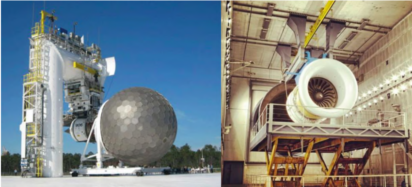
Figure 2.2: Exterior (left) and interior (right) test cells [17].
