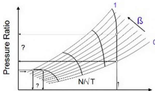
Figure 4.12: Generic compressor map with \beta -lines [11].
