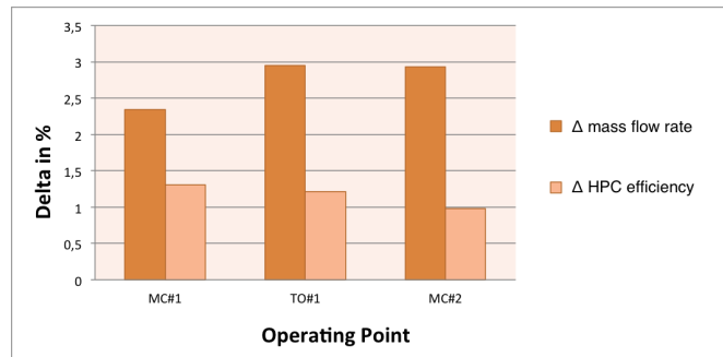
Figure 5.6: Variation of HPC efficiency and capacity.
