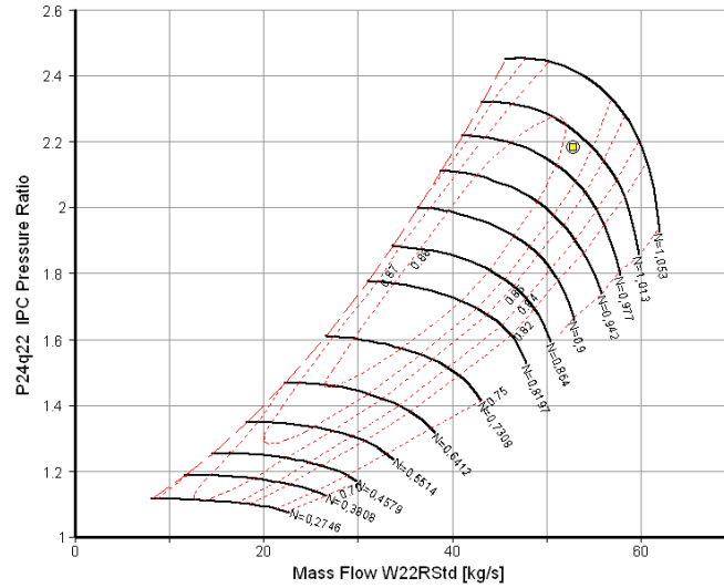
Figure 4.13: Booster map.
