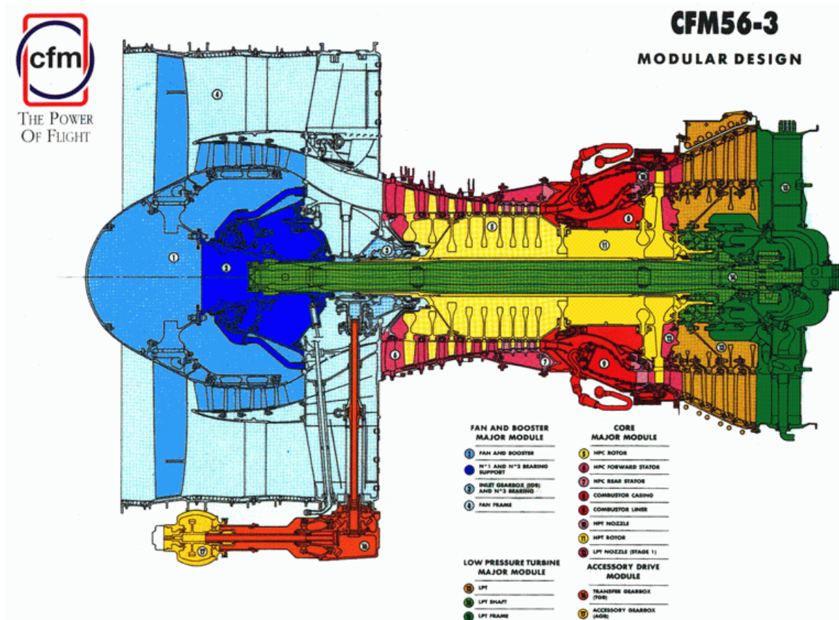
Figure 4.1: CFM56-3 schematic [22].
