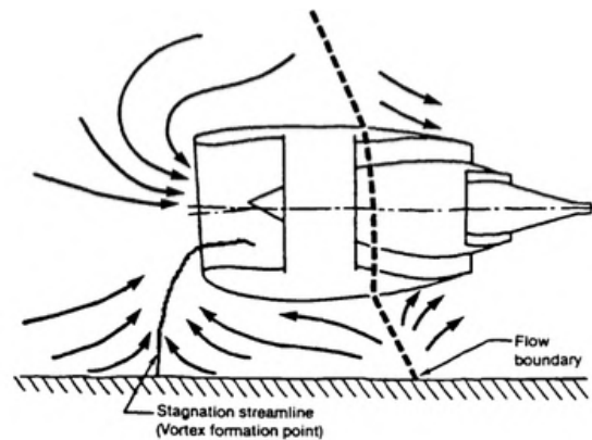
Figure 3.5: Dust ingestion in a turbine due to ground vortex formation [33].
