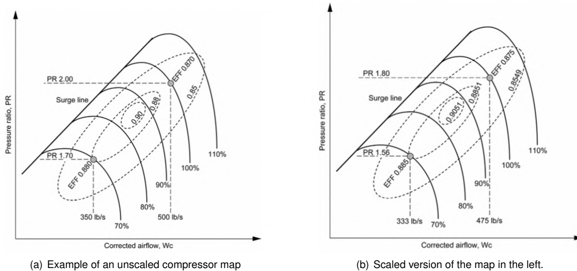
Figure 4.10: Scaling of compressor map [45].
