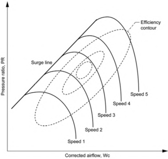
Figure 4.9: Generic compressor map [45].
