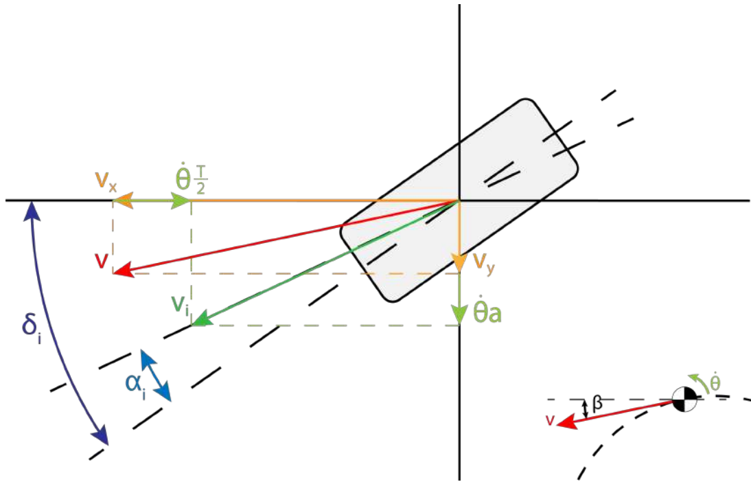
Figure 2.2: Geometric reference variables
