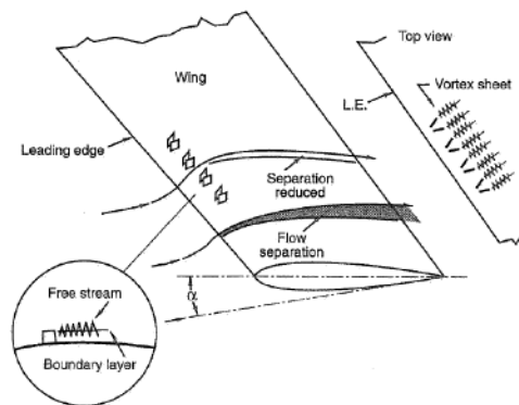
Figure 15.57 Vortex generator.
