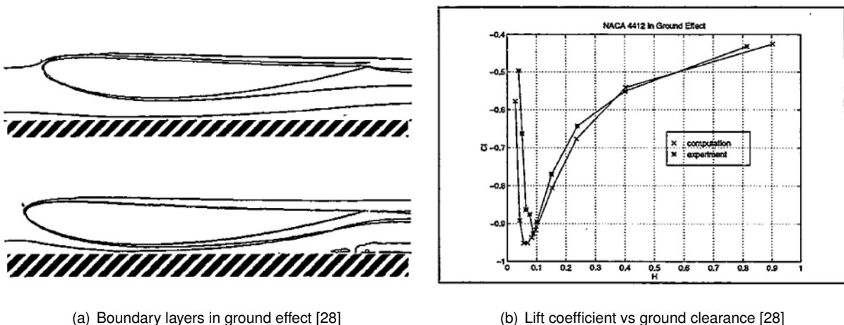
Figure 2.12: Ground effect
