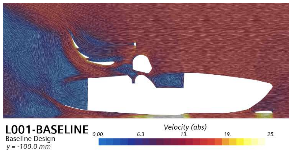
Figure 3.13: Airflow speed at y=-100\text{mm}
