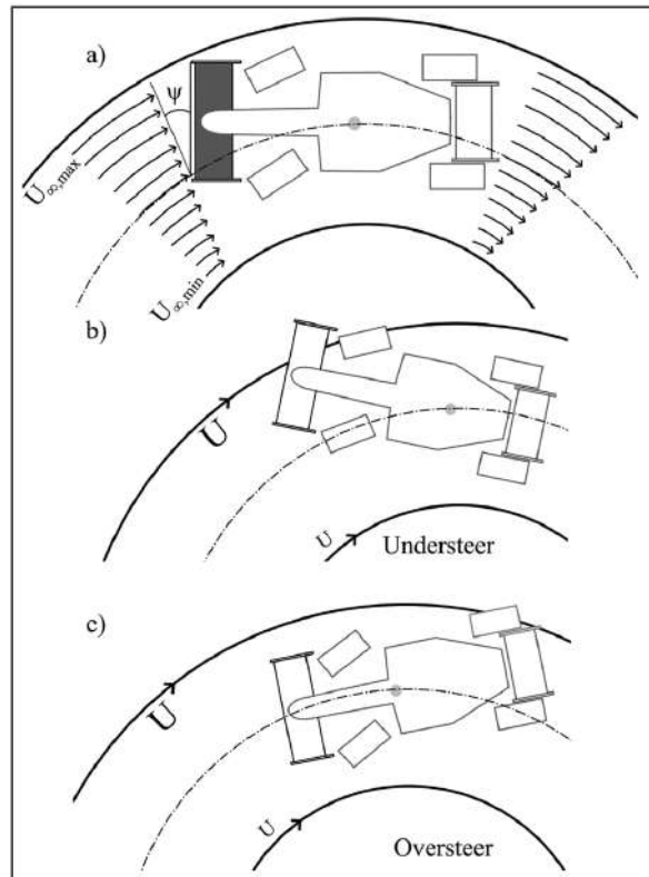
Figure 2.7: Understeer and oversteer [14]
