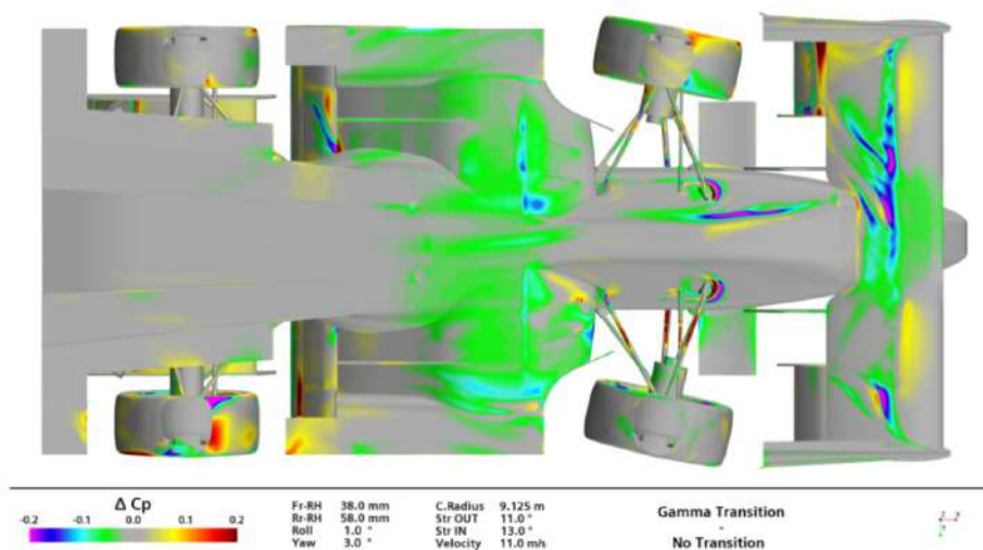
Figure 2.30: Transition study
