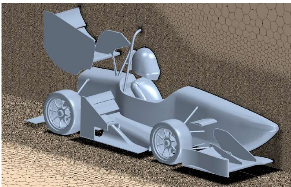
Figure 3.2: Mesh
