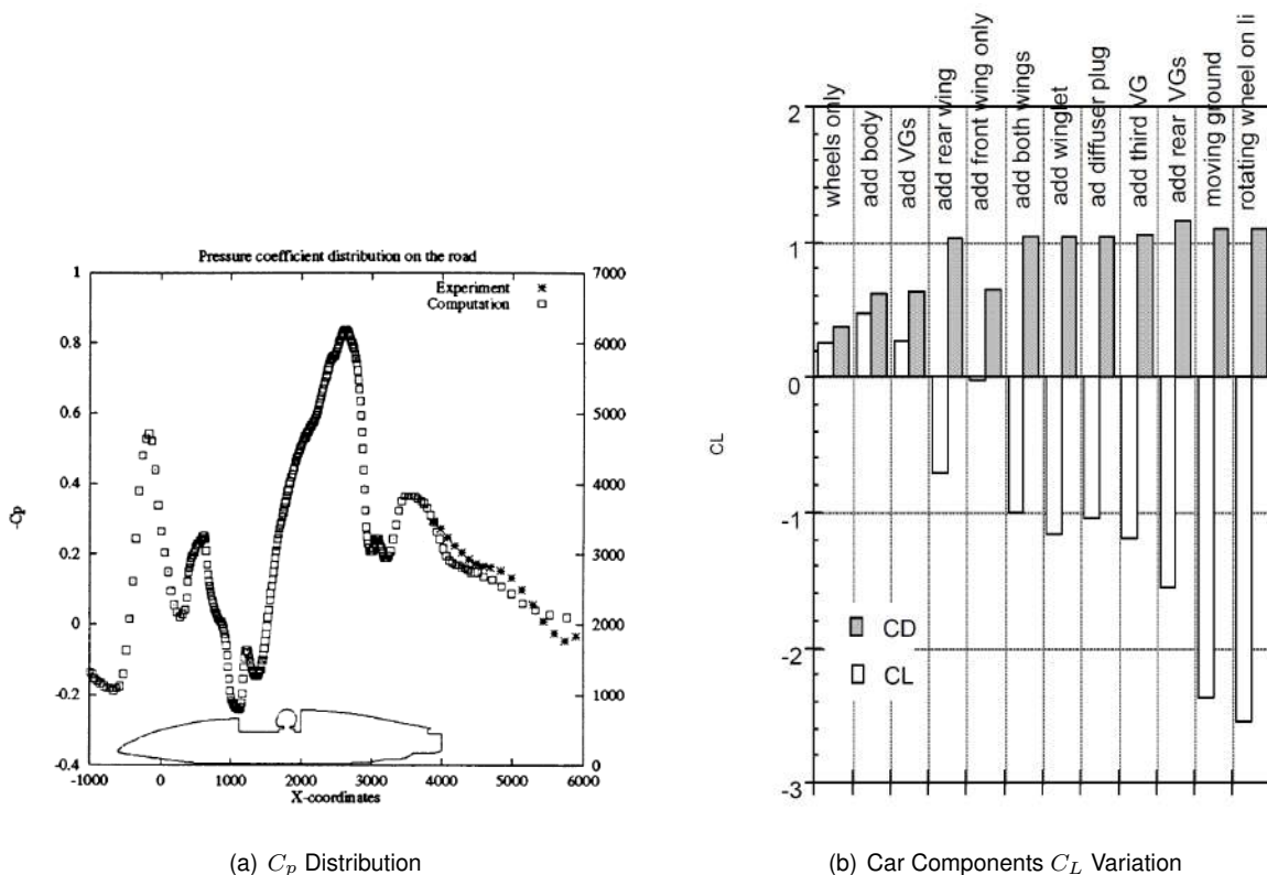
Figure 2.24: Pressure Variation [40]
